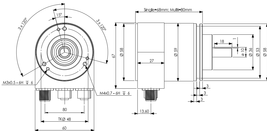
Clamp Flange (F)
