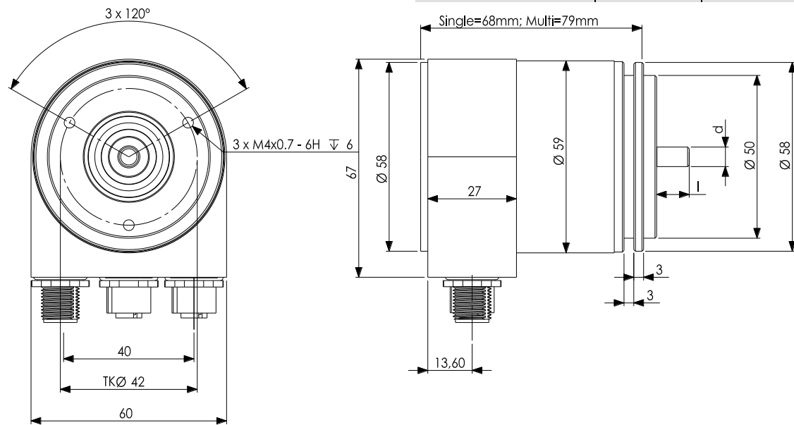
Clamp Flange (F)
